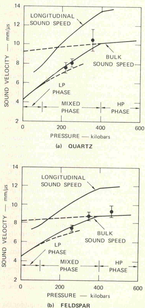
Fig. 4. Hugoniot sound velocities measured in quartz and feldspar. Approximate locations of phase boundaries on the Hugoniot are indicated. Solid lines show the estimated bulk and longitudinal sound velocity in the low-pressure, mixed, and high-pressure phase regions. Dashed lines are metastable extensions of the estimated sound velocity out of the stability field of the low- and high-pressure phases, respectively.
